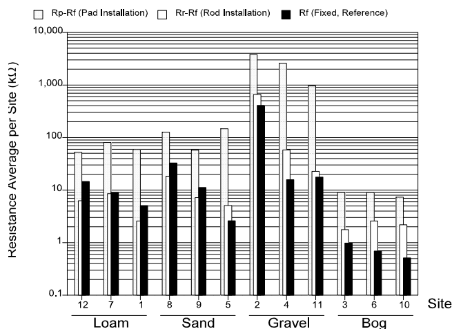
Figure 9. Comparison of installation contact resistance to fixed electrode spreading/contact resistance.
