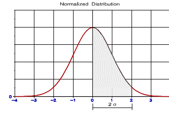
Figure 3. Upper tail (shaded) of the 95% confidence interval.
