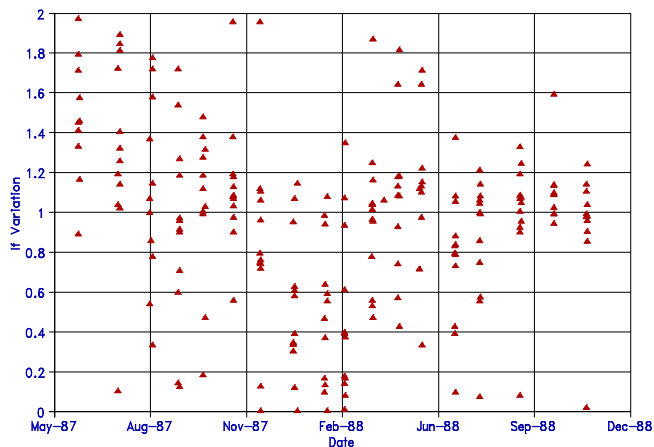
Figure 6. Fixed-electrode current data variation for all 12 sites and over 18 months.
