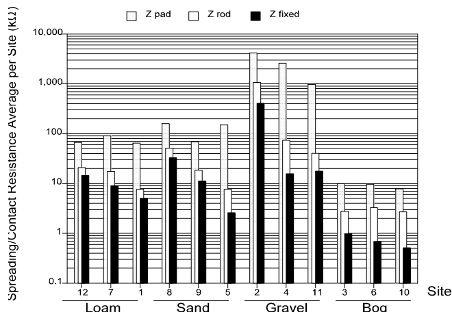
Figure 8. Comparison of spreading/contact resistance for various probe designs and deployments.
